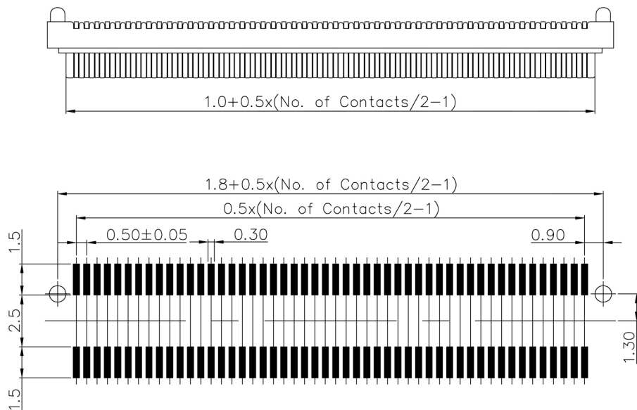
PCB Layout For Surface Mounting
