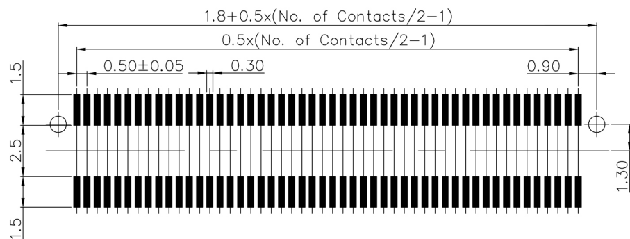
PCB Layout For Surface Mounting
