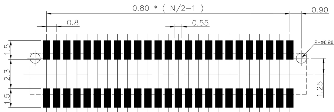
PCB Layout For Surface Mounting
