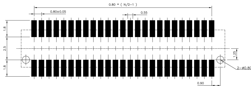
PCB Layout For Surface Mounting
