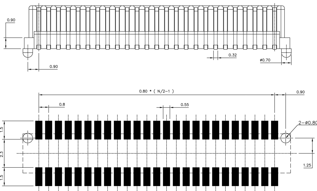
PCB Layout For Surface Mounting
