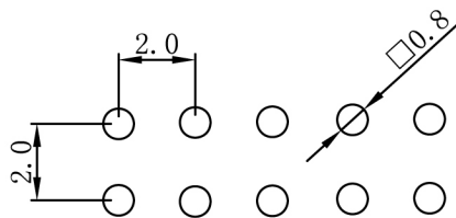
P. C. B Hole Layout
