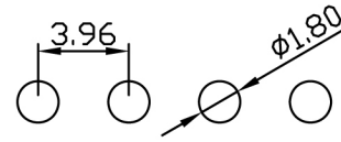
P. C. B Hole Layout
